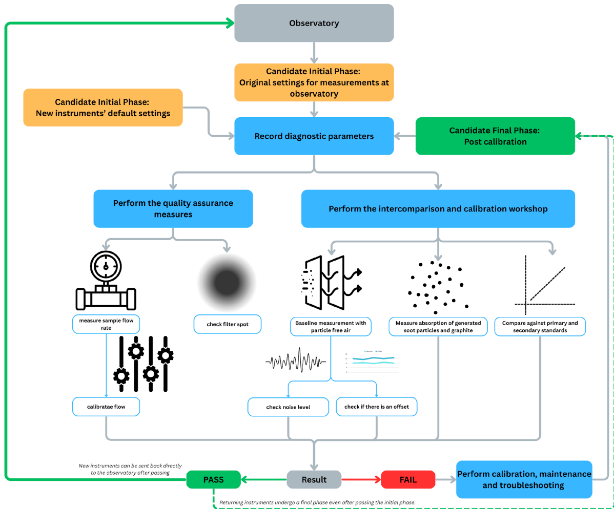
Figure 4 Schematic diagram of the recommended calibration and intercomparison procedures performed at the facility for the measurement of Abs using a FAP.
